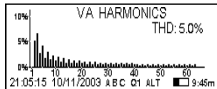
View THD and individual harmonics through the front panel display screen
